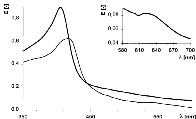
Fig. 3. Absorption spectrum of purified CP from Bacillus SF. Thick line, 9 μM native enzyme; thin line, the cyano-adduct obtained by the addition of 25 mM KCN to the native enzyme. Inset is an expanded scale of the visible portion of the spectrum. Experimental conditions were as described in Materials and methods
